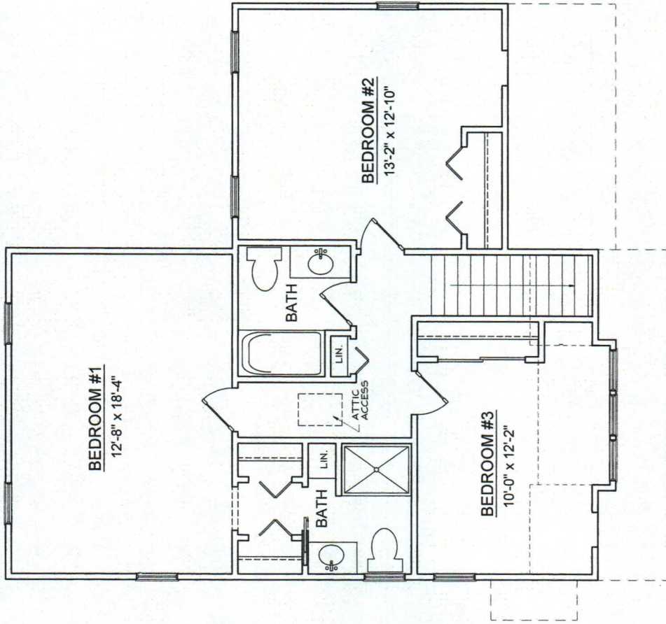
Second Floor 874 square feet
